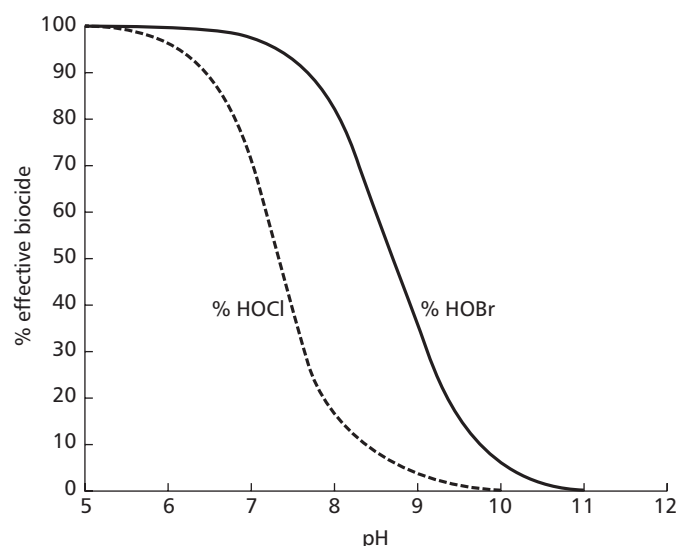
Figure 11 Relationship between effective free chlorine or bromine and pH
