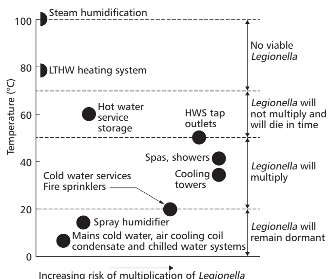
Figure 2 System design/operating temperatures and multiplication of Legionella
