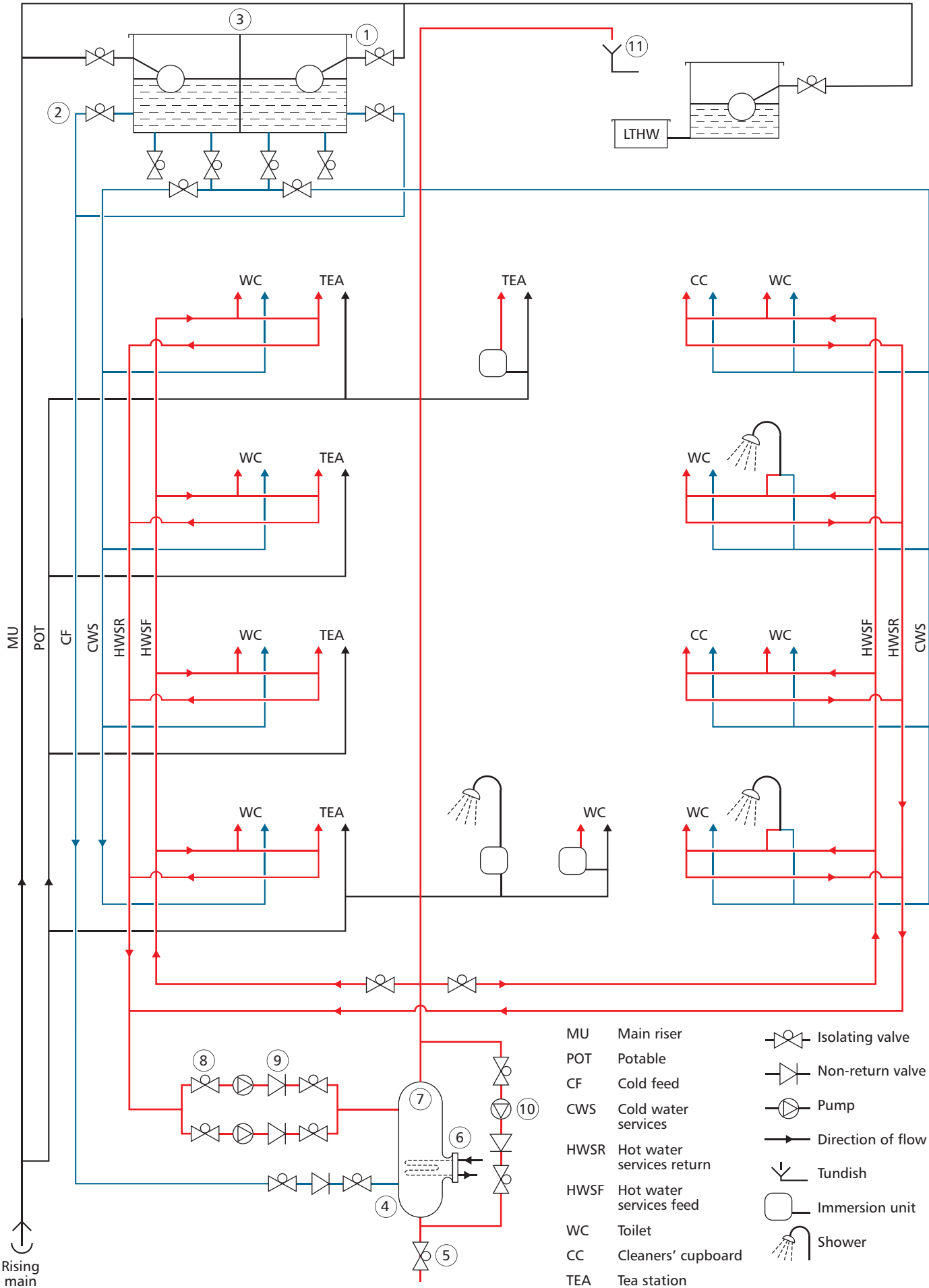
Figure 13 Example hot water system for a large office (For notes see Table 6)
