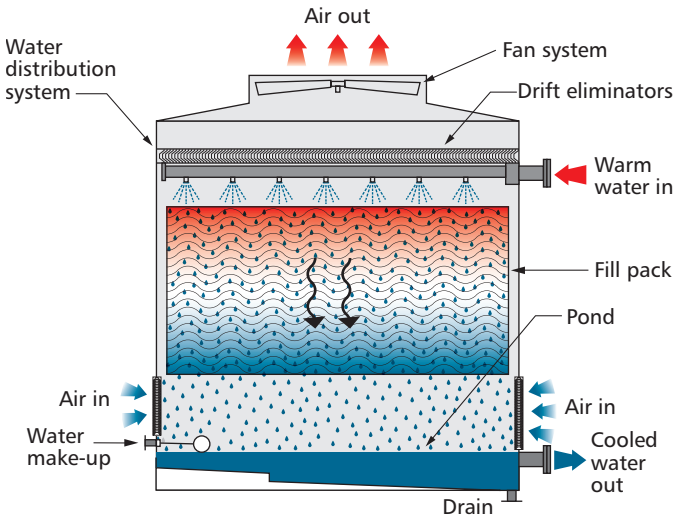
Figure 3 Components of an induced draught counter-flow cooling tower
