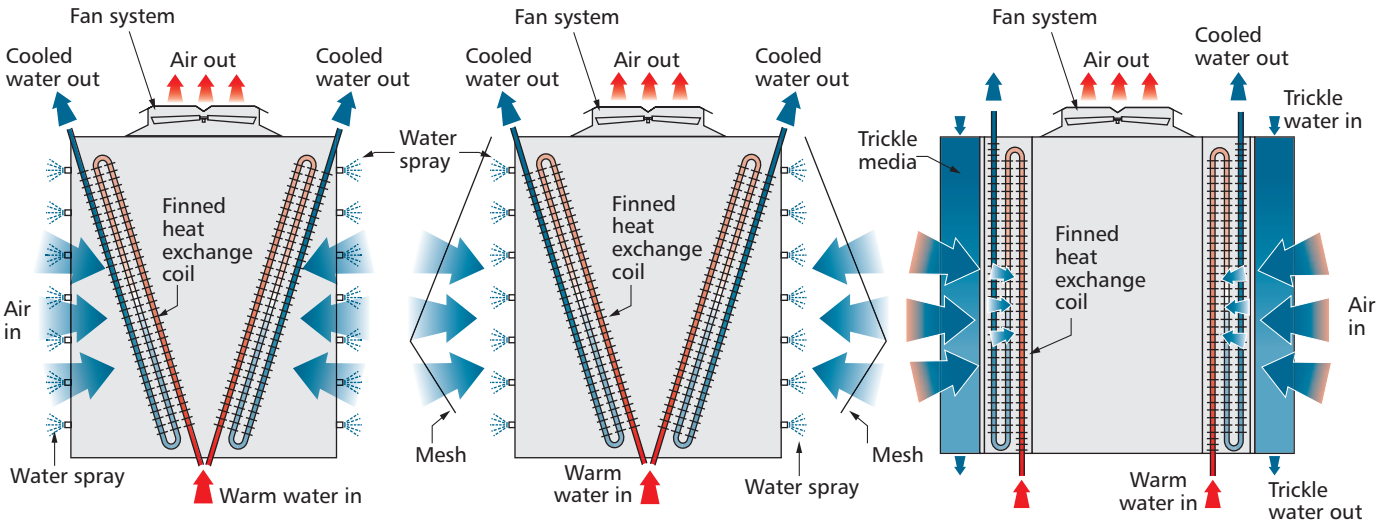
Figure 8 Three types of adiabatic coolers
